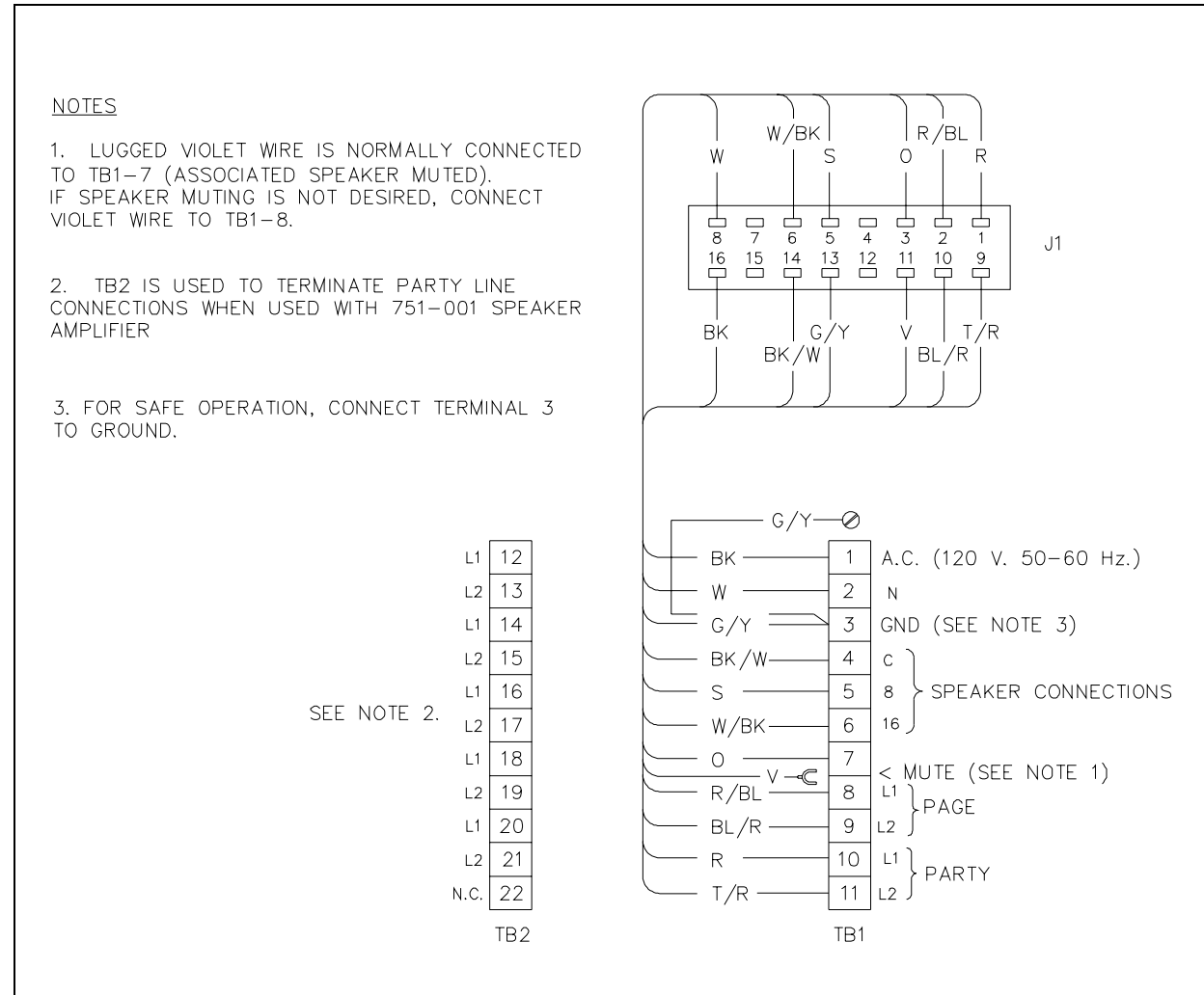
Figure 2. Wiring Diagram
