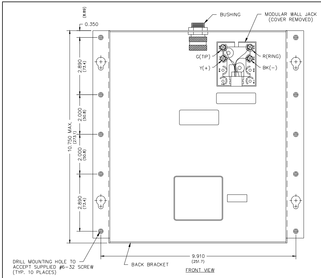
Figure 2. Model 295F Modular Wall Jack Wiring and Back Box Mounting Details
