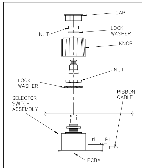
Figure 1. Knob Assembly View
