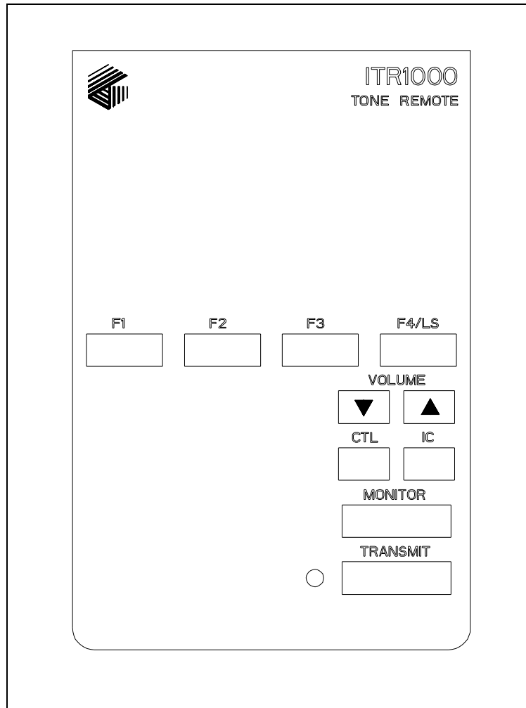
Front View of the ITR1000-001 Desk Set Button Panel
