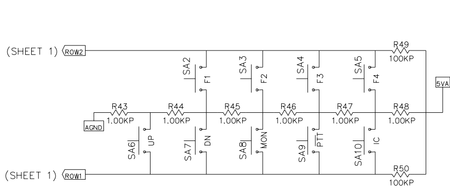
Tone Desk Set I/O Section Schematic Diagram - Sheet 2
