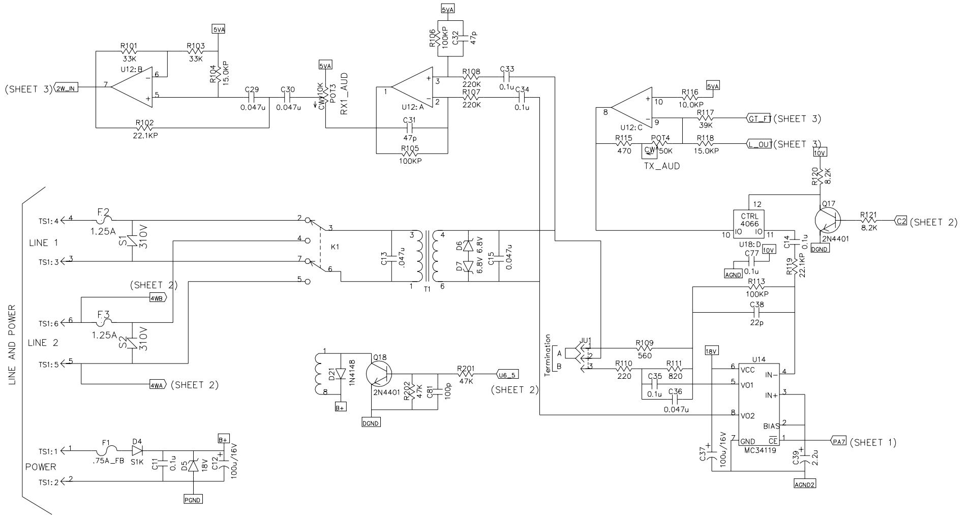
Tone Desk Set Audio Section 2 Schematic Diagram - Sheet 4
