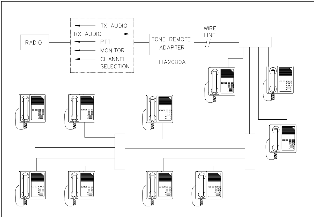
Sample ITR1000-001 Installation Diagram - Shown connected in parallel within one building.
