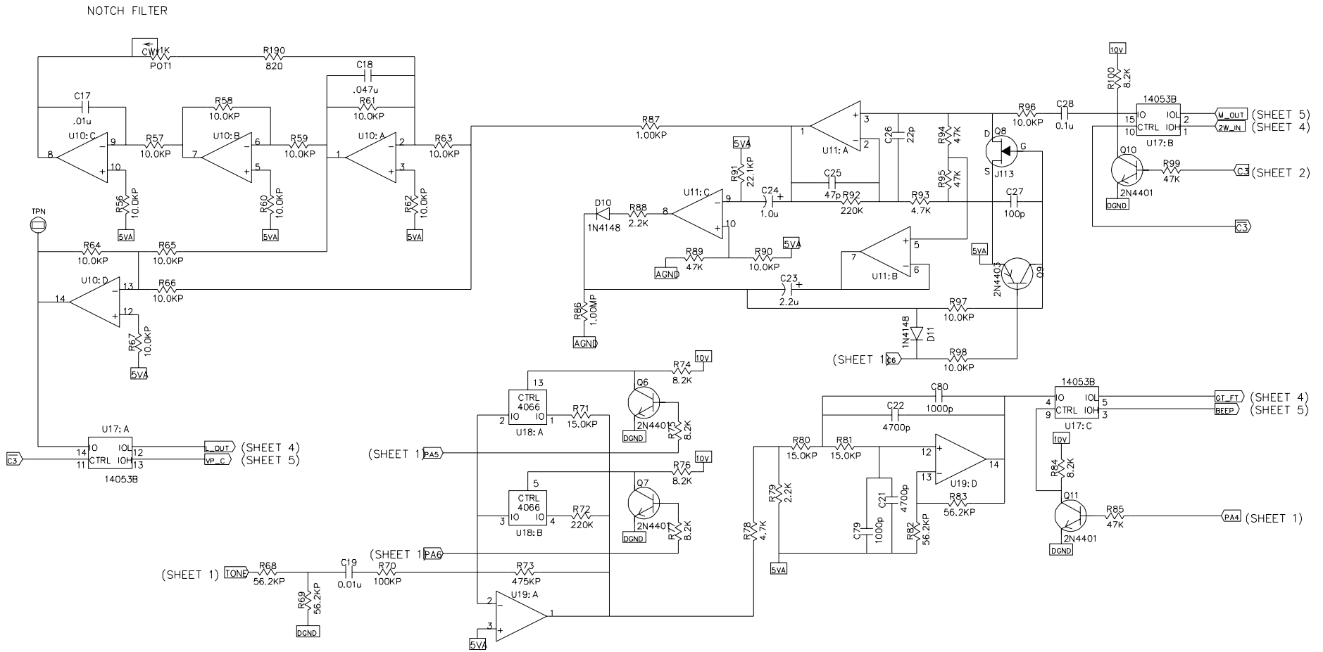
Tone Desk Set Audio Section 1 Schematic Diagram - Sheet 3
