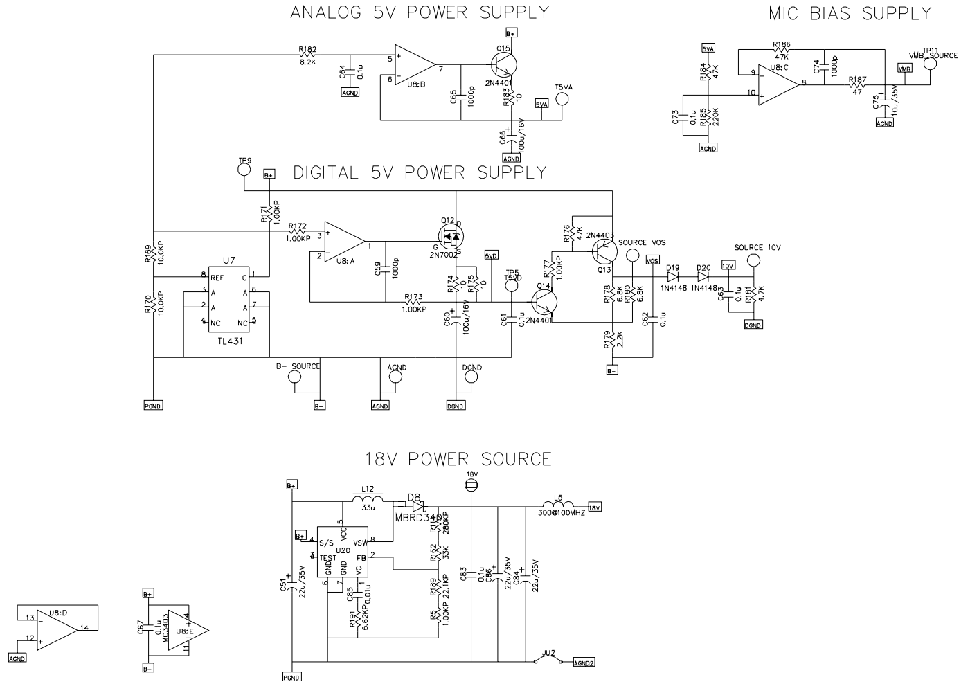
Tone Desk Set Power Supply Schematic - Sheet 6
